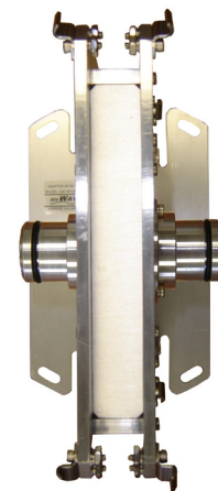
Four slots at antenna attachment points allow \pm 3^\circ polarization adjustment.
